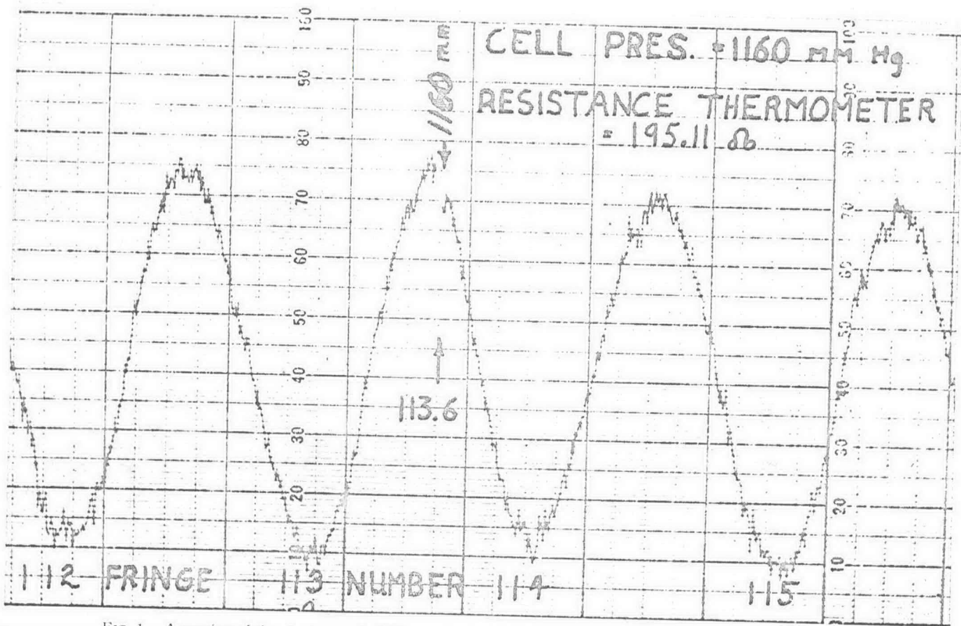
FIG. 1. A portion of the chart record of fringes obtained during the 3.000^{\circ}\text{K} \mu - P compressibility isotherm.
